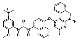
1-[4-(2-Benzylamino-6-methyl-pyrimidin-4-yloxy)-naphthalen-1-yl]-3-(5-tert-butyl-2-methoxy-phenyl)-urea;
